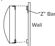
Typical Side View
