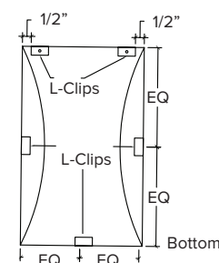
Vertical - Rear View
