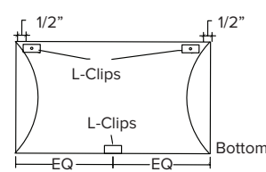
Horizontal - Rear View
