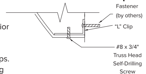
Vertical - Rear View
