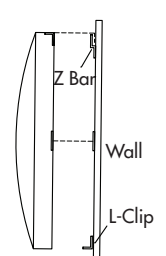
VERTICAL - SIDE VIEW
